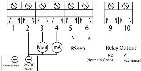
FIGURE 4: WIRING
