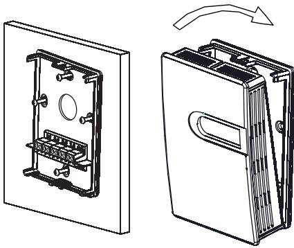
FIGURE 3: BACKPLATE
