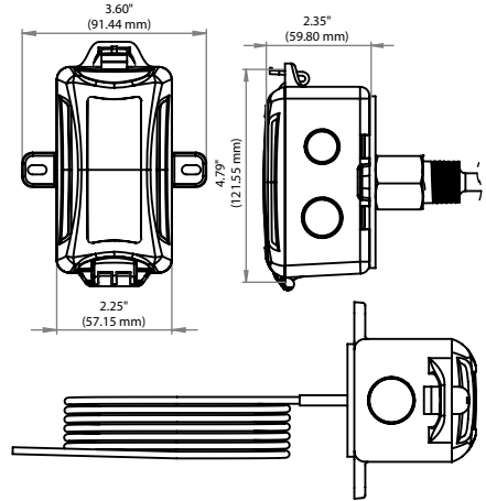
FIGURE 1: ENCLOSURE DIMENSIONS
