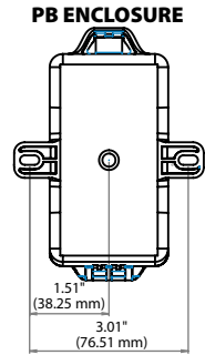
FIGURE 4: MOUNTING CLIP DIMENSIONS
