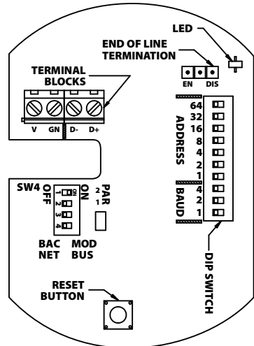
FIGURE 2: LAYOUT
