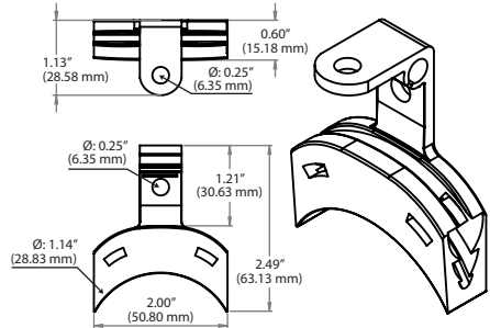
UNIVERSAL PLASTIC MOUNTING CLIP (ACI #145421)
