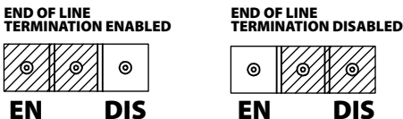
FIGURE 6: EOL TERMINATION JUMPERS
