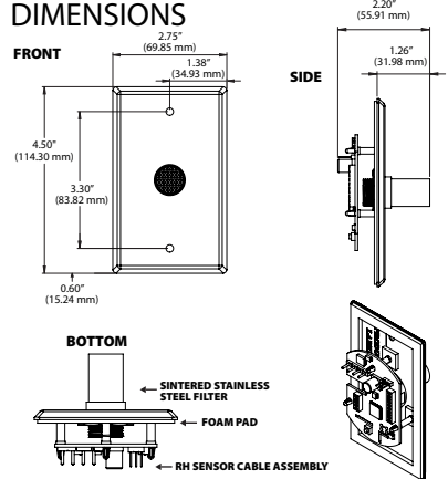
FIGURE 1: ENCLOSURE DIMENSIONS
