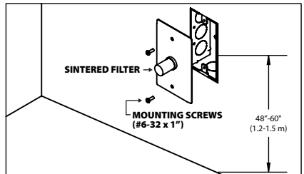
FIGURE 2: MOUNTED ASSEMBLY
