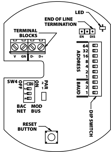
FIGURE 4: LAYOUT
