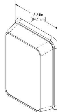
BAPI-Stat "Quantum" Enclosure (with optional 60mm mounting base for European wall boxes)
