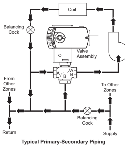
Figure-7 Typical Primary-Secondary Piping.
