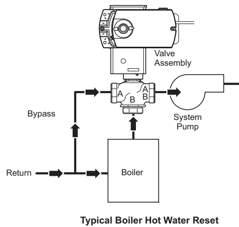
Figure-6 Typical Boiler Hot Water Reset.
