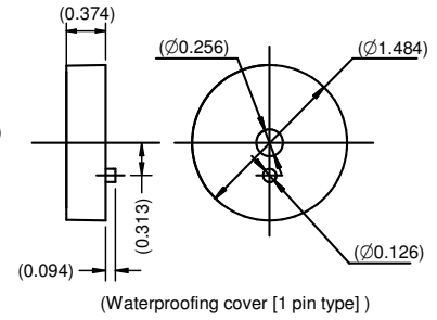
(Waterproofing cover [1 pin type])
