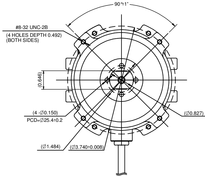
(Waterproofing cover [1 pin type])
