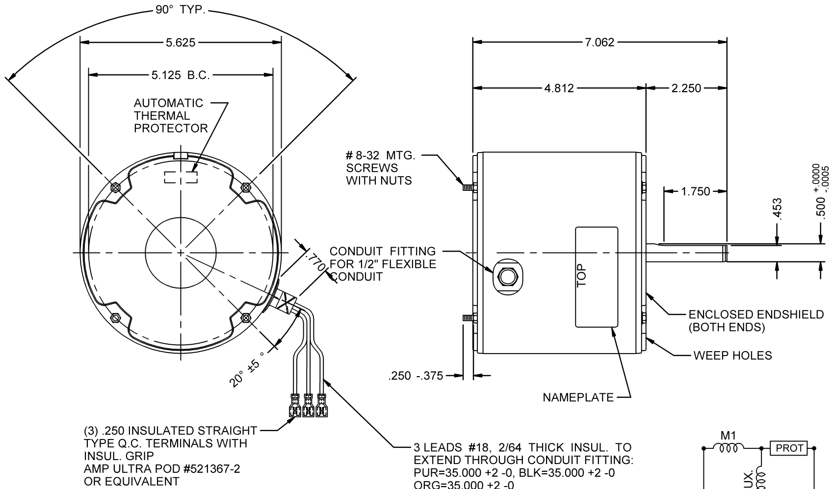
MOTOR MOUNTED IN SHAFT-DOWN POSITION
