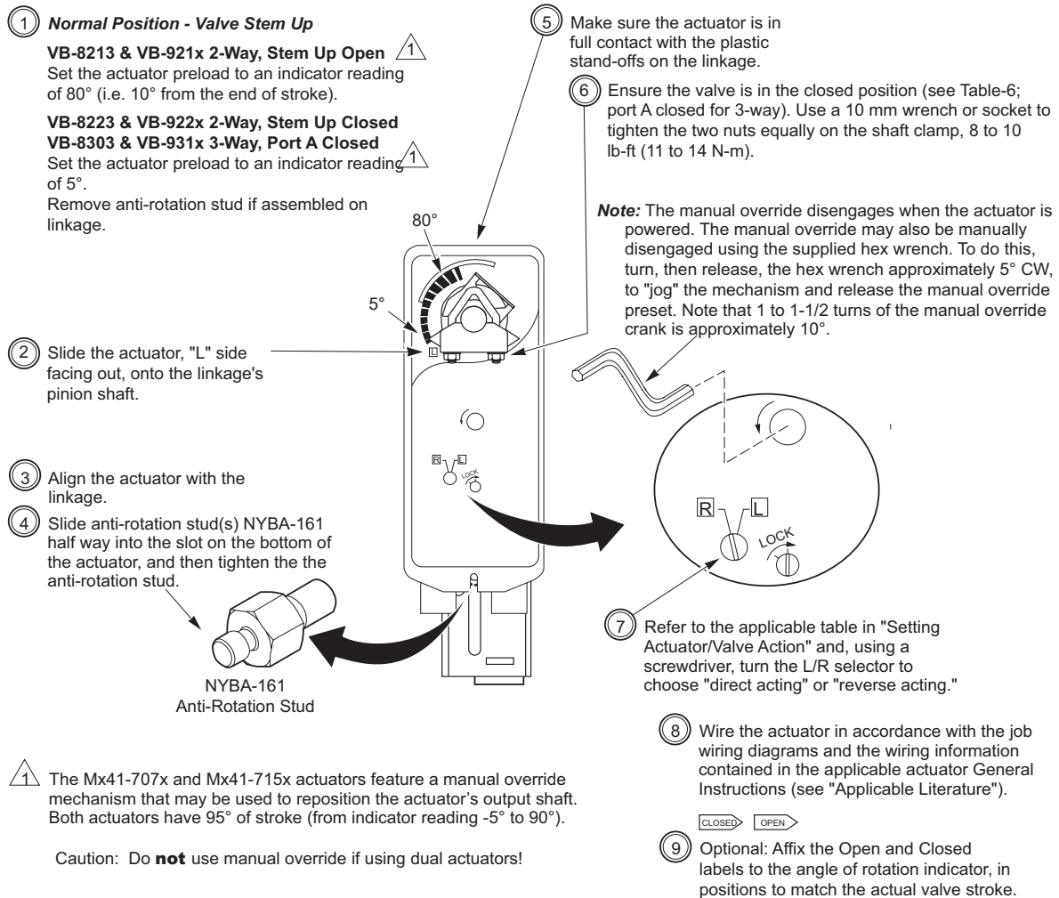
Figure-4 Mounting Mx41-707x or Mx41-715x and Setting Up Actuator/Linkage/Valve
