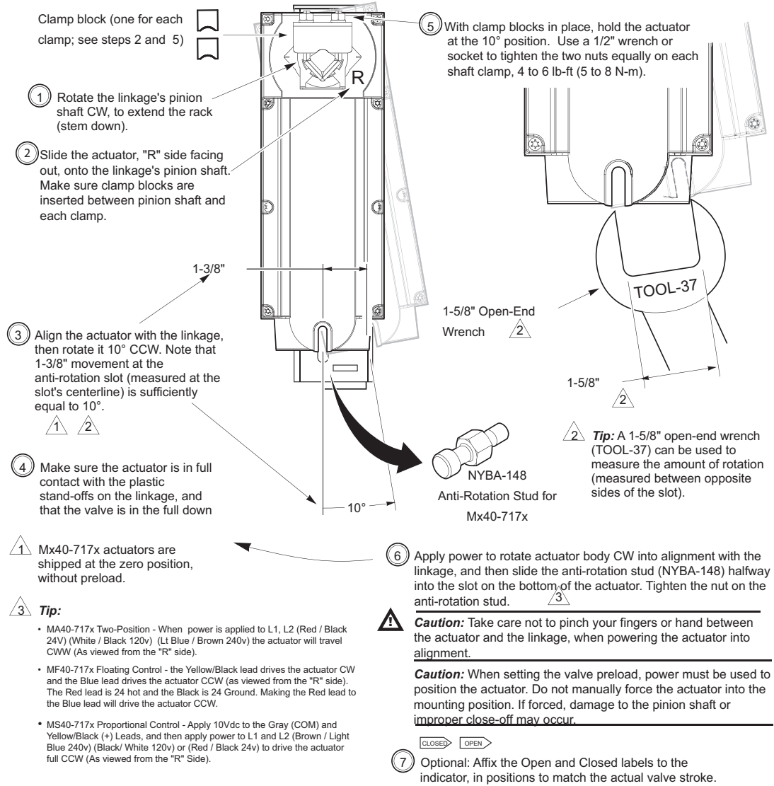
Figure-8 Mounting Mx40-717x and Setting Up Actuator/Linkage/Valve
