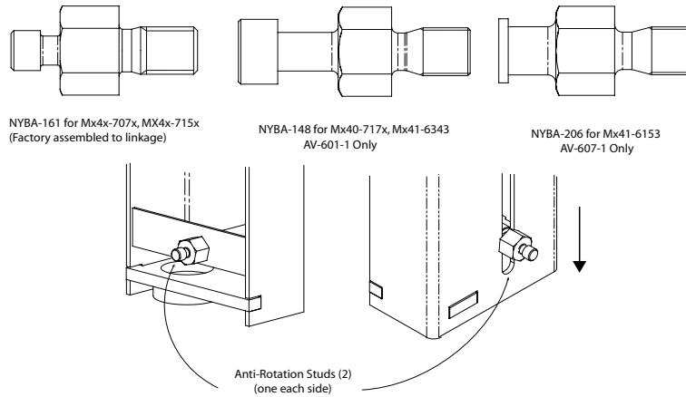
Figure-2 Anti-Rotation Studs
