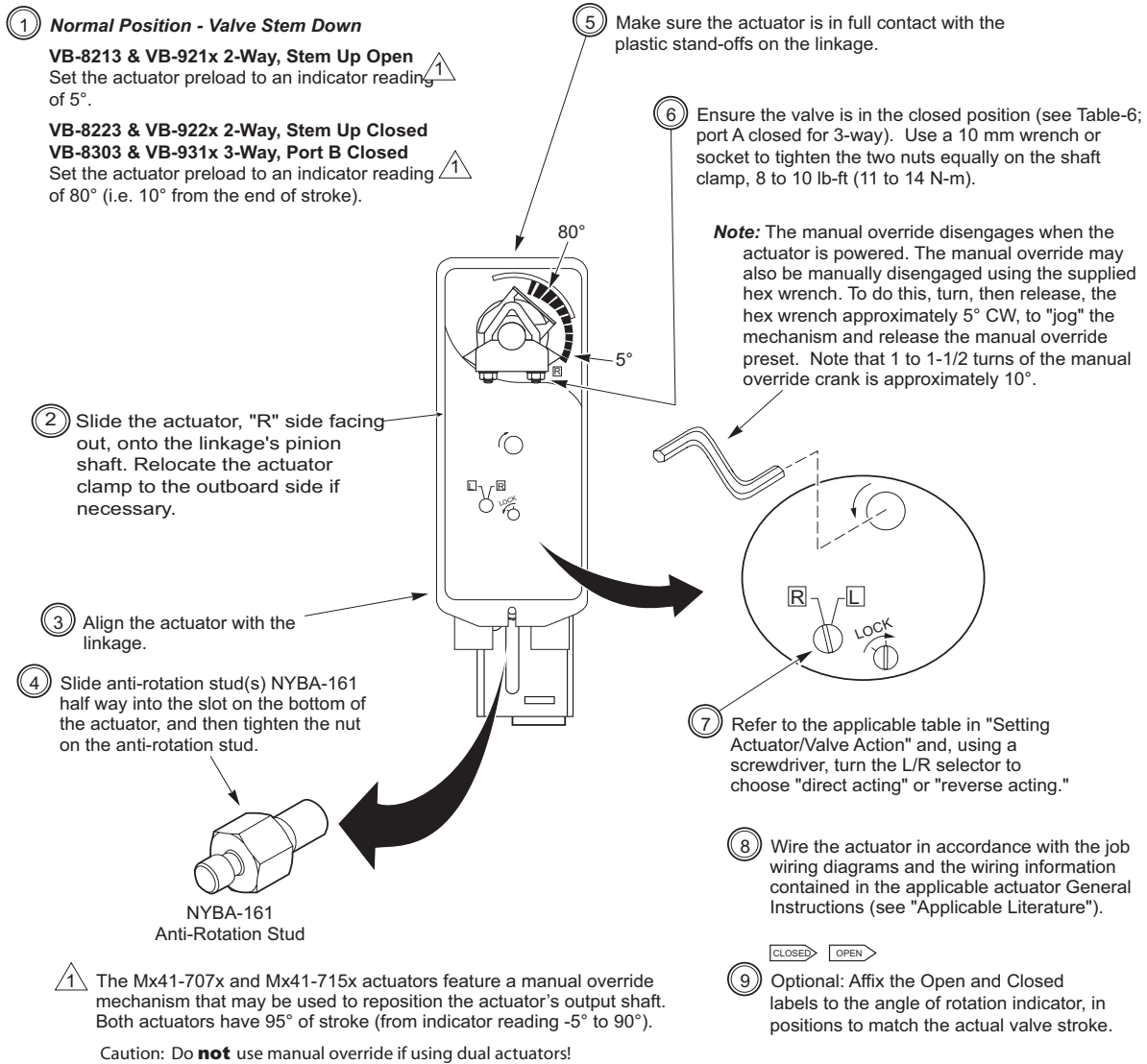
Figure-5 Mounting Mx41-707x or M41-715x and Setting Up Actuator/Linkage/Valve
