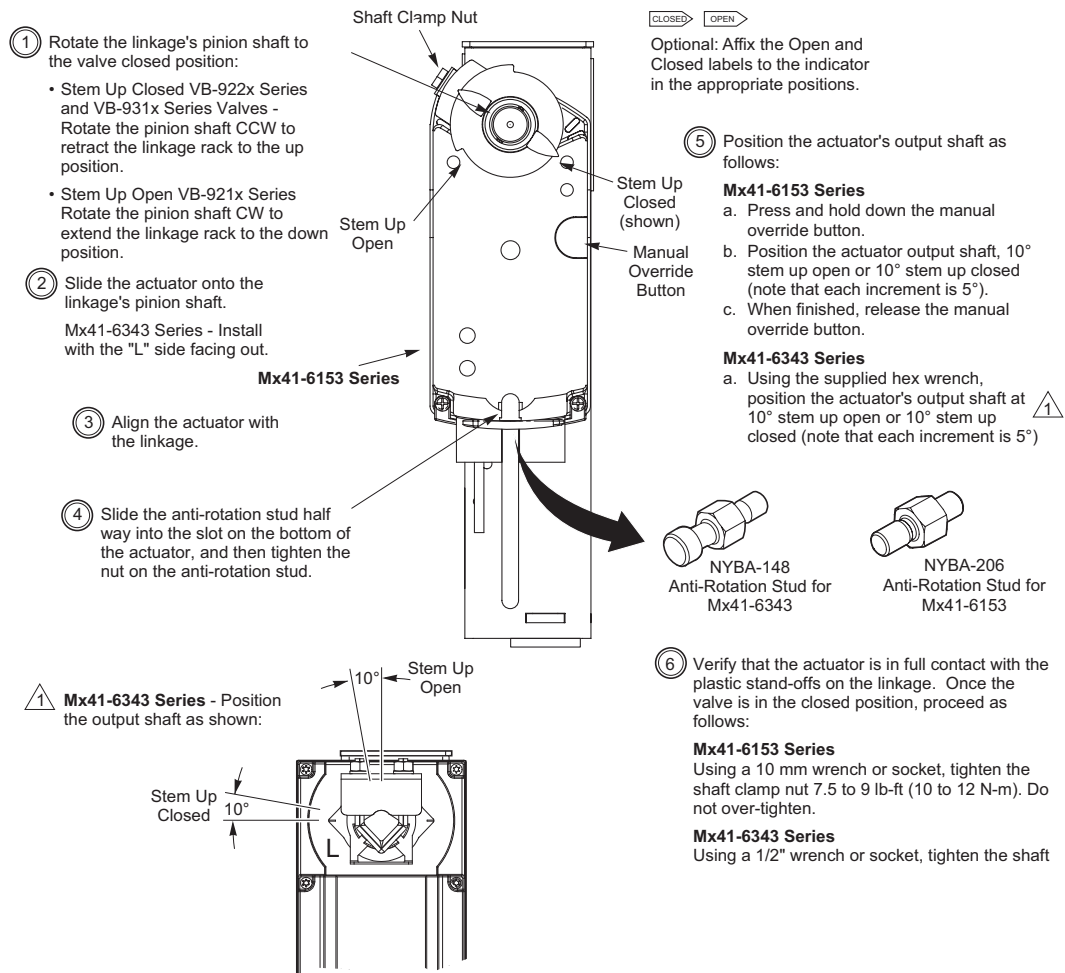
Figure-6 Mounting Mx41-6153 Series or Mx41-634x Series Actuator and Setting Up Actuator/Linkage/Valve
