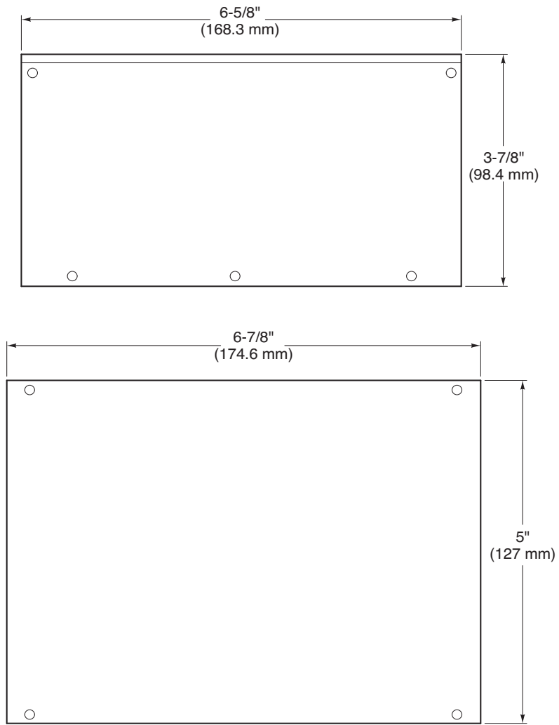
Figure-2 AM-369 Gasket Cover Kit Dimensions.
