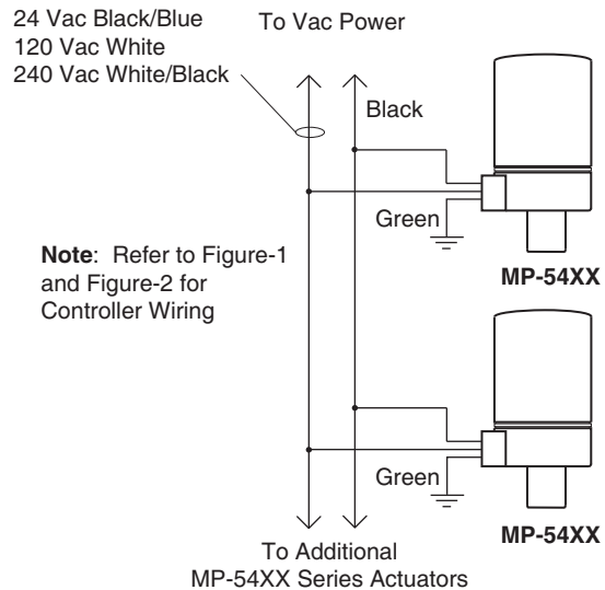
Figure-4 Wiring of Multiple MP-5400 Series Actuators to Single Power Source.
