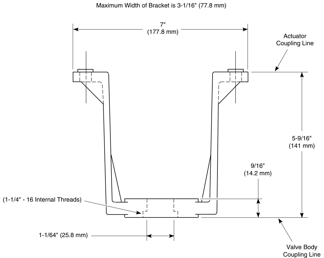
Figure-8 Dimensions of the Valve Linkage Mounting Bracket.
