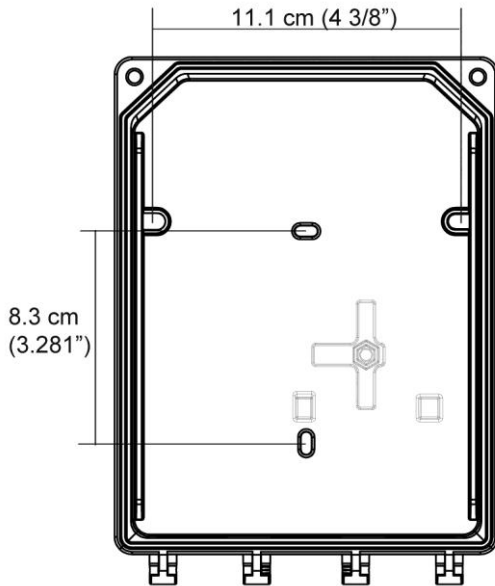
Figure 1. Unit Dimensions
