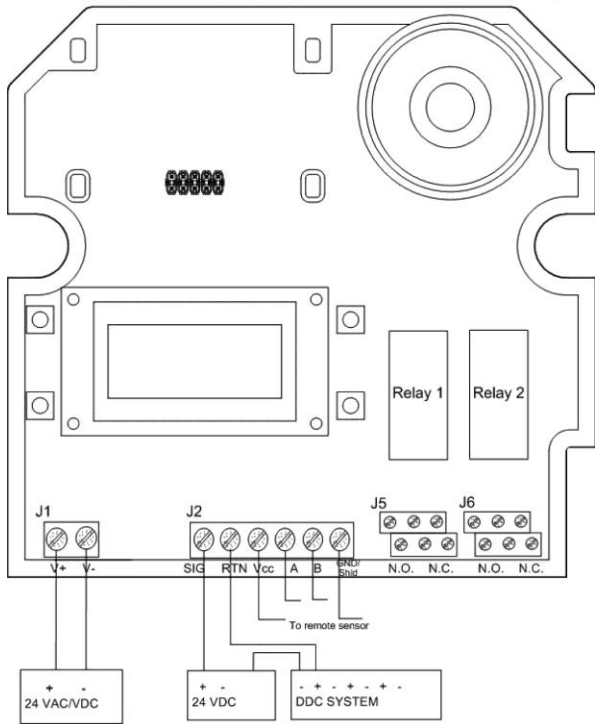
Figure 5. 4-Wire Current Sink Output
