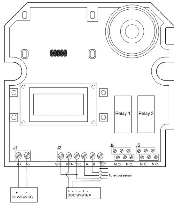
Figure 4. 4-Wire Current Source Output
