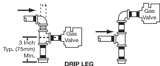
DRIP LEG
